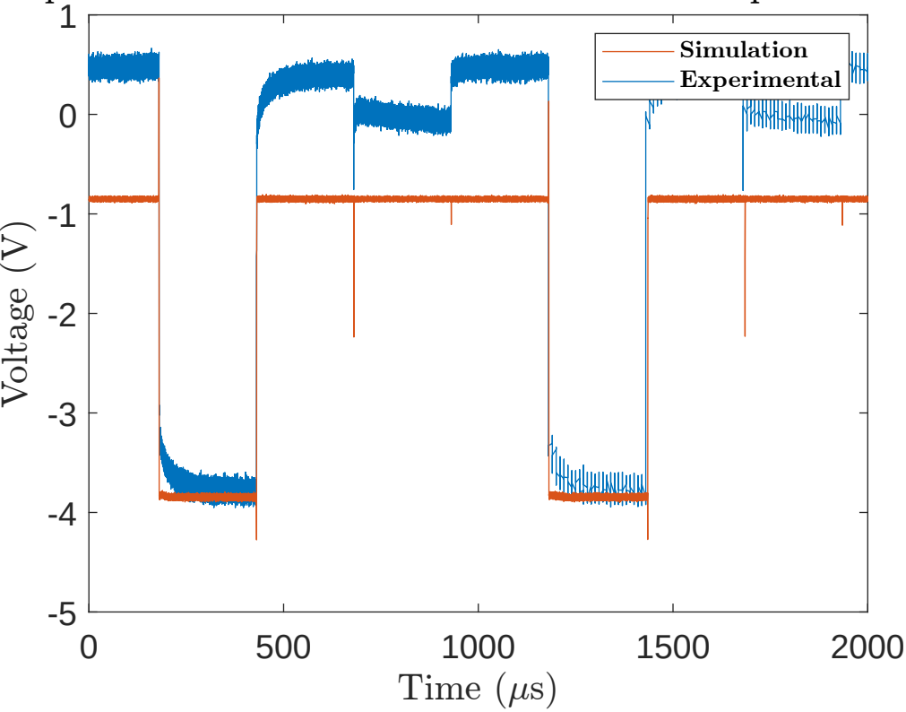
Experimental and Simulated NAND Gate Output at 2 kHz
