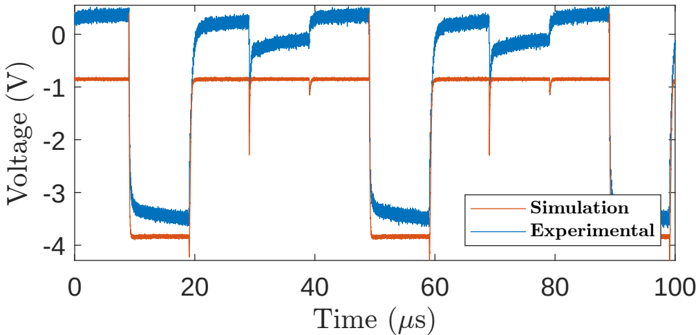
Experimental and Simulated NAND Gate Output at 50 kHz
