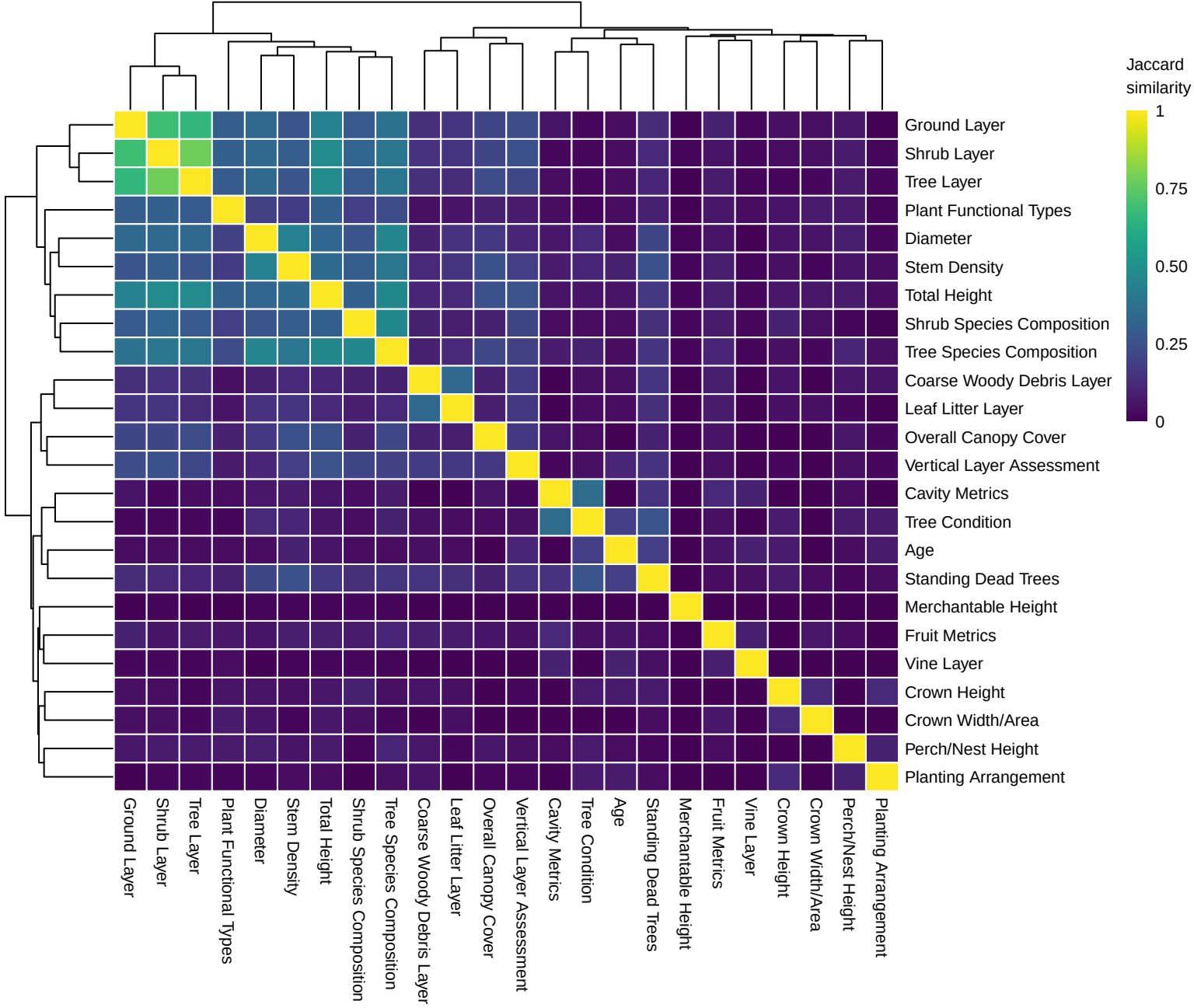
Avian: Metric Co-occurrence (Jaccard Similarity)
