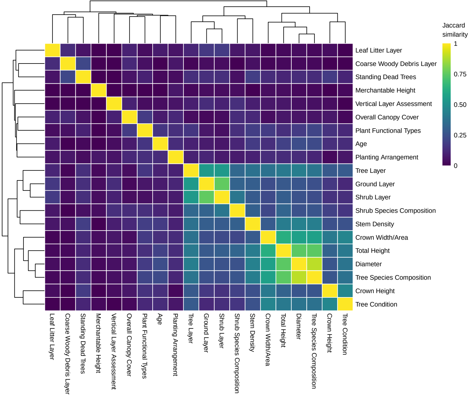
Carbon: Metric Co-occurrence (Jaccard Similarity)
