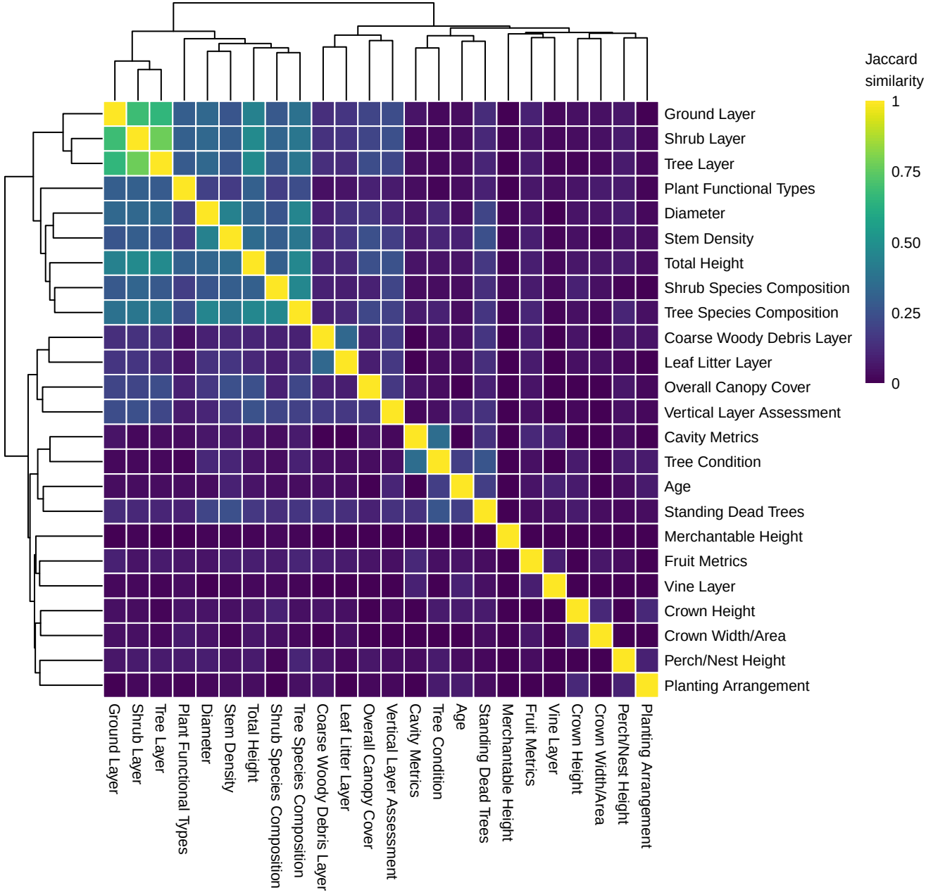
Avian: Metric Co-occurrence (Jaccard Similarity)
