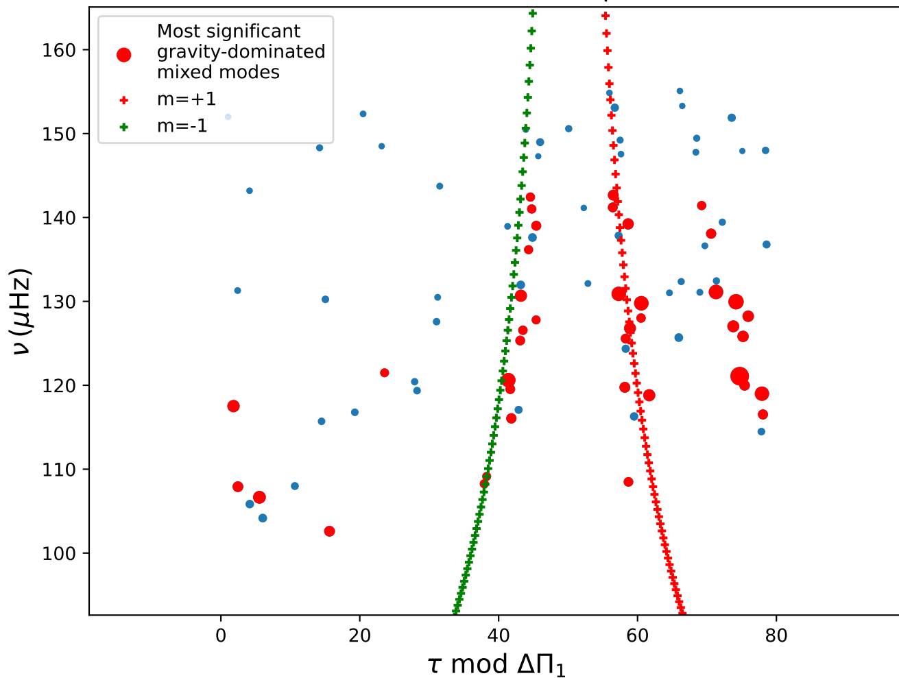
KIC 6144777 with \Delta\Pi_1 = 79.10 s: fit with 2 rotational components
