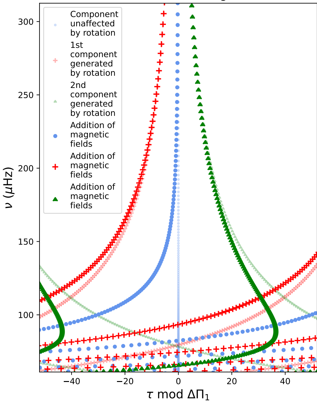
Synthetic échelle diagram showing the effects of rotation and magnetic fields
