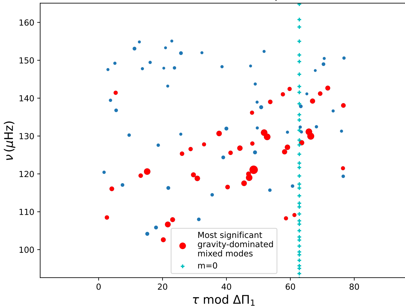
KIC 6144777 with \Delta\Pi_1 = 76.80 s: fit with 1 rotational component
