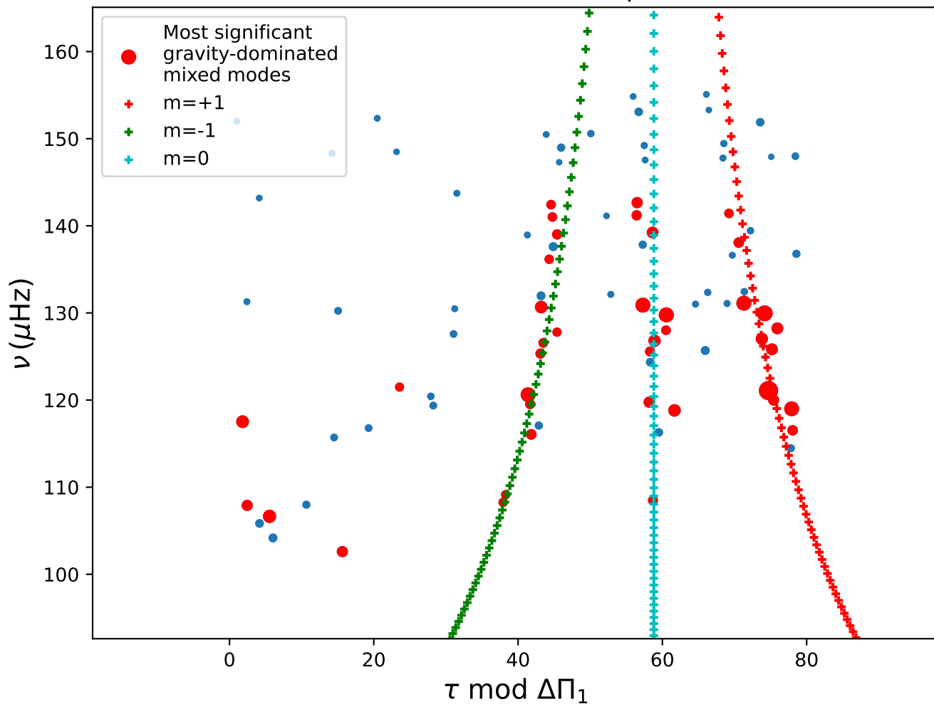
KIC 6144777 with \Delta\Pi_1 = 79.10 s: fit with 3 rotational components
