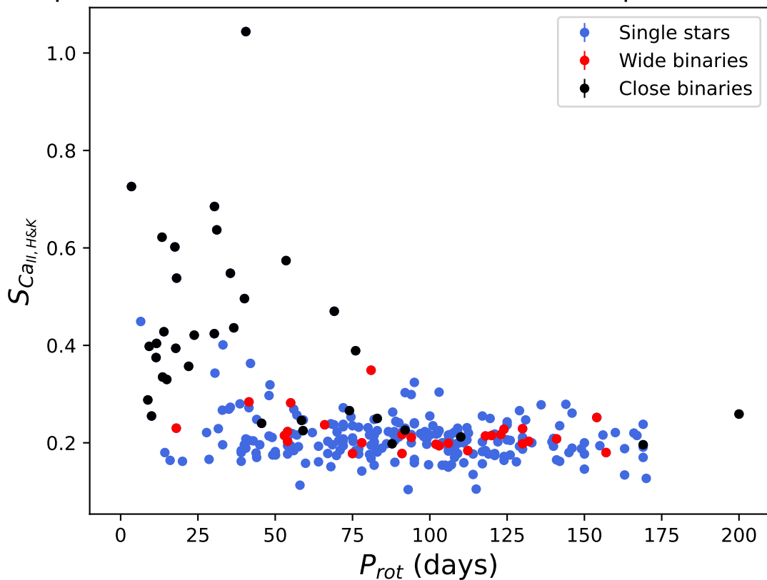
Level of magnetic activity as probed by the CaII H&K spectral lines as a function of the rotation period of stars
