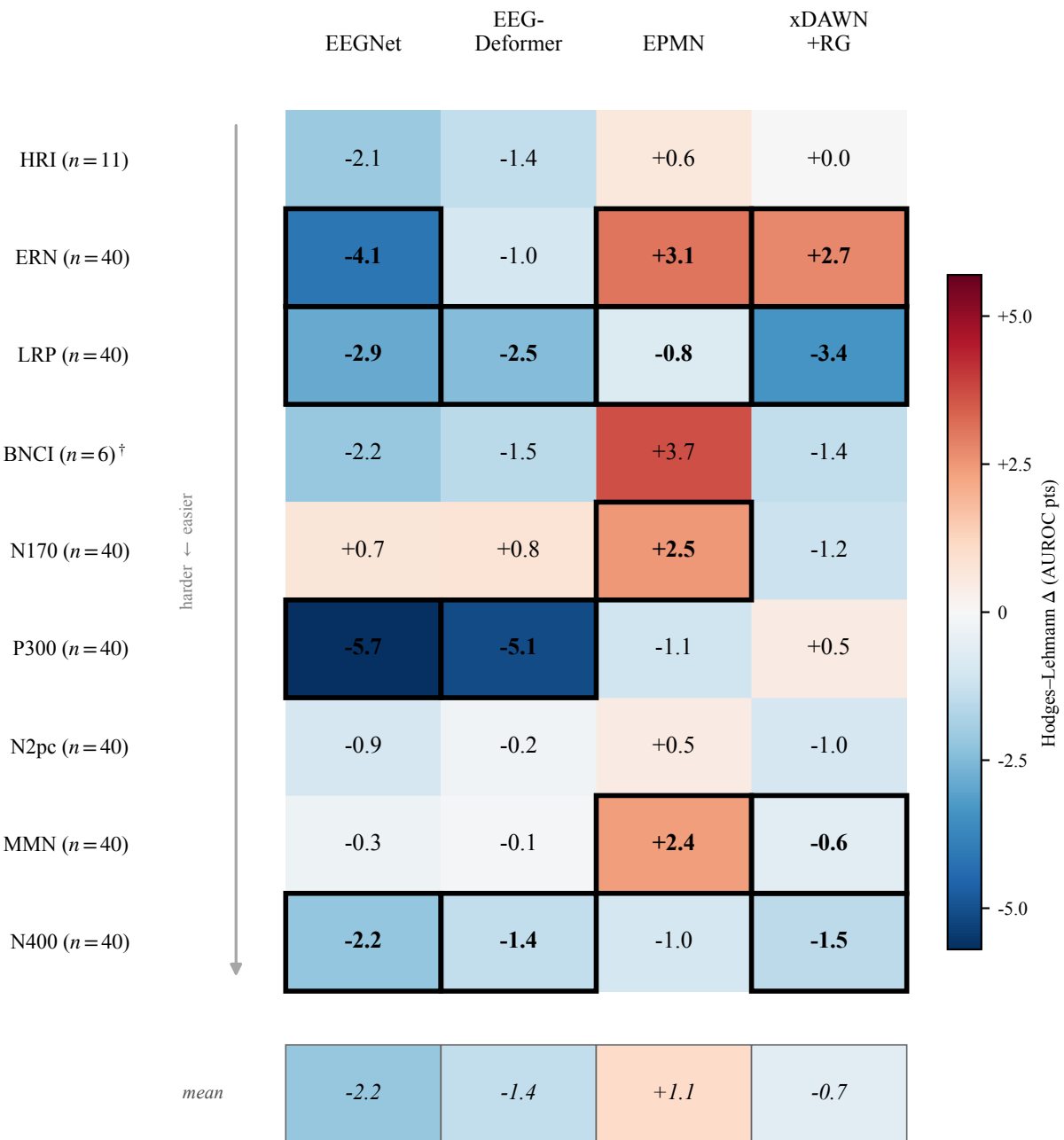
Paired Advantage of ERP-XTTN vs Baselines (3-Channel)
