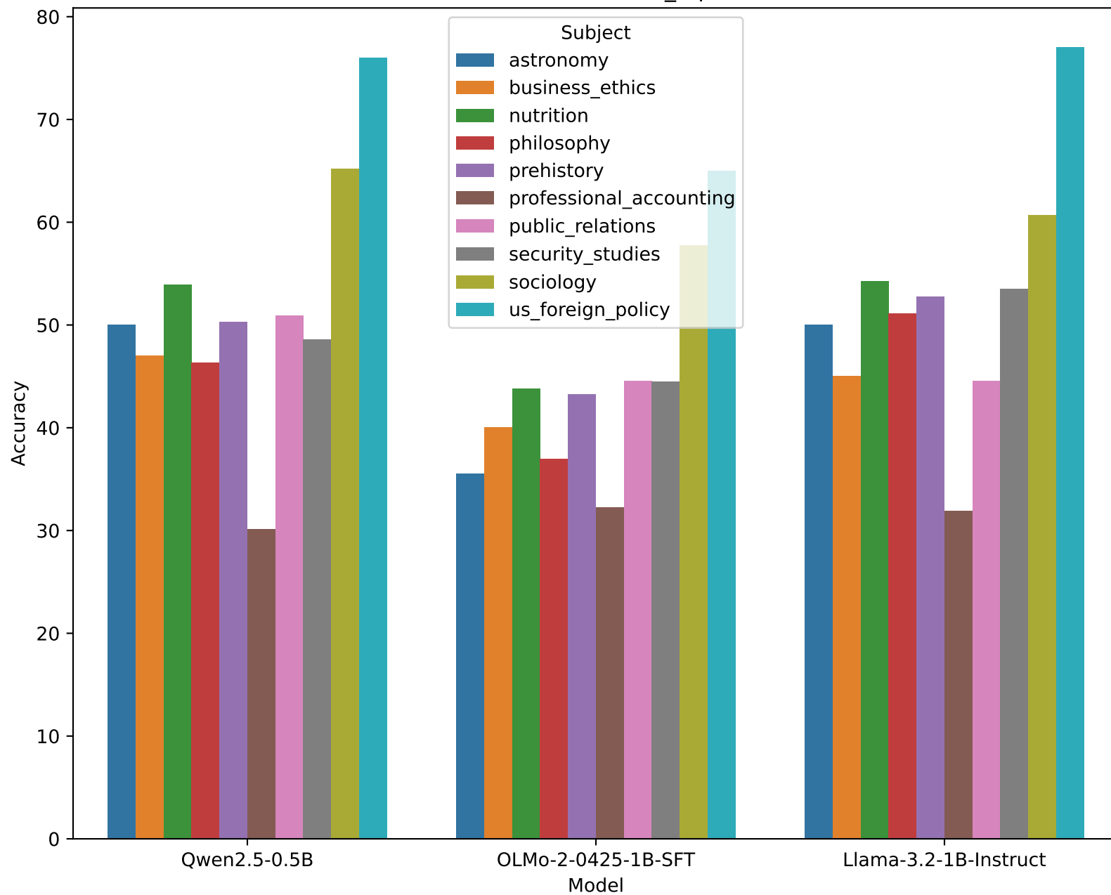
MMLU Results full_mps
