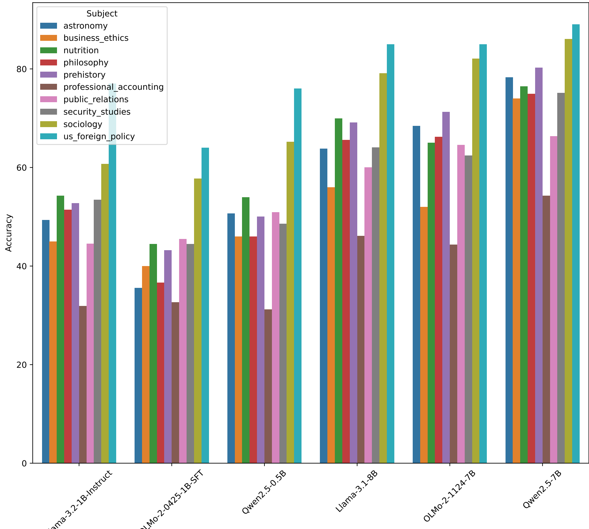
MMLU Results full_cuda
