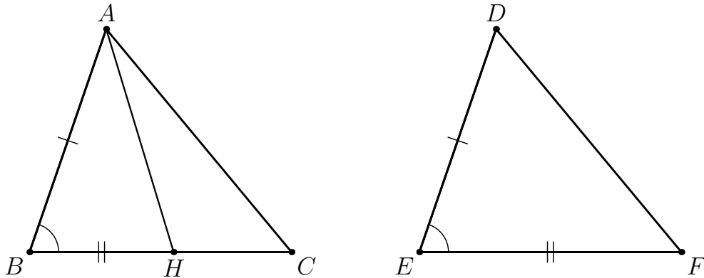
Figure 3: Euclid's SAA reductio configuration. The point H lies between B and C . The diagram marks exactly the local SAS data AB \cong DE , BH \cong EF , and \angle ABH \cong \angle DEF . Proposition I.16 is then applied to \triangle AHC .
