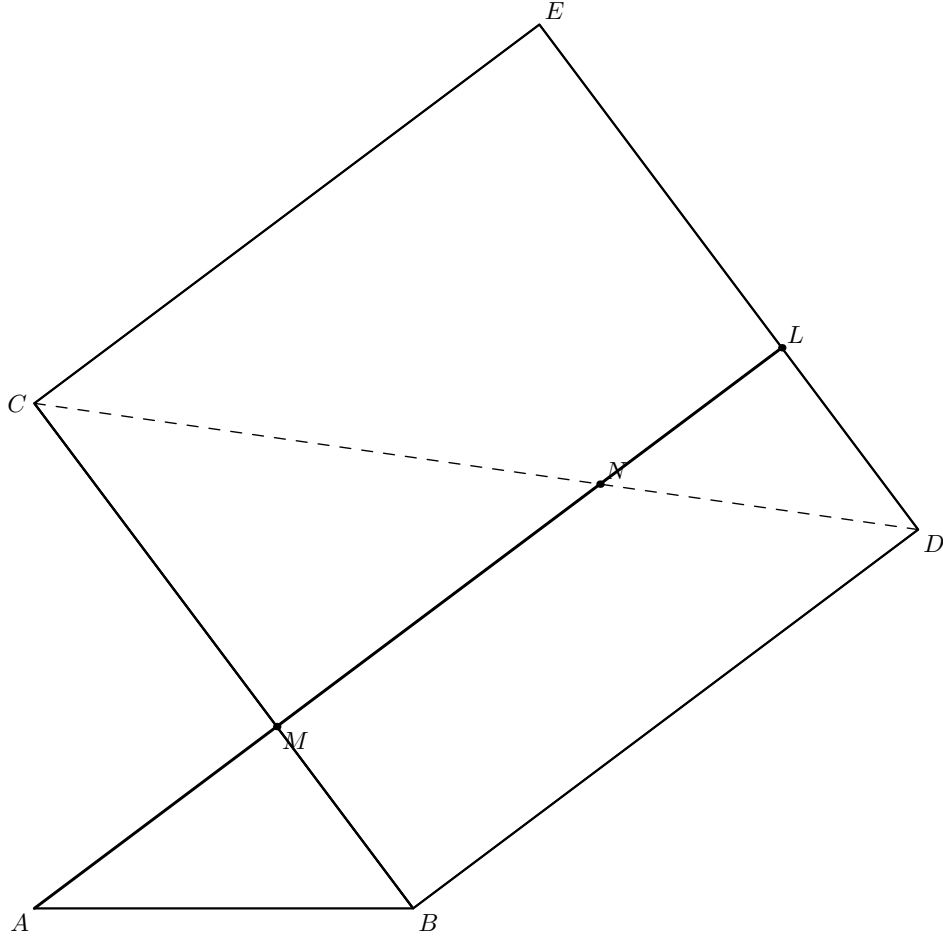
Figure 2: The internal cut constructed by i47_cut_core . The perpendicular foot satisfies B - M - C . Completing C, E, M gives the parallelogram CELM , carrier uniqueness puts A, M, L on one line and D, L, E on the opposite side of the square, and forced Pasch supplies N with D - N - C and M - N - L .
