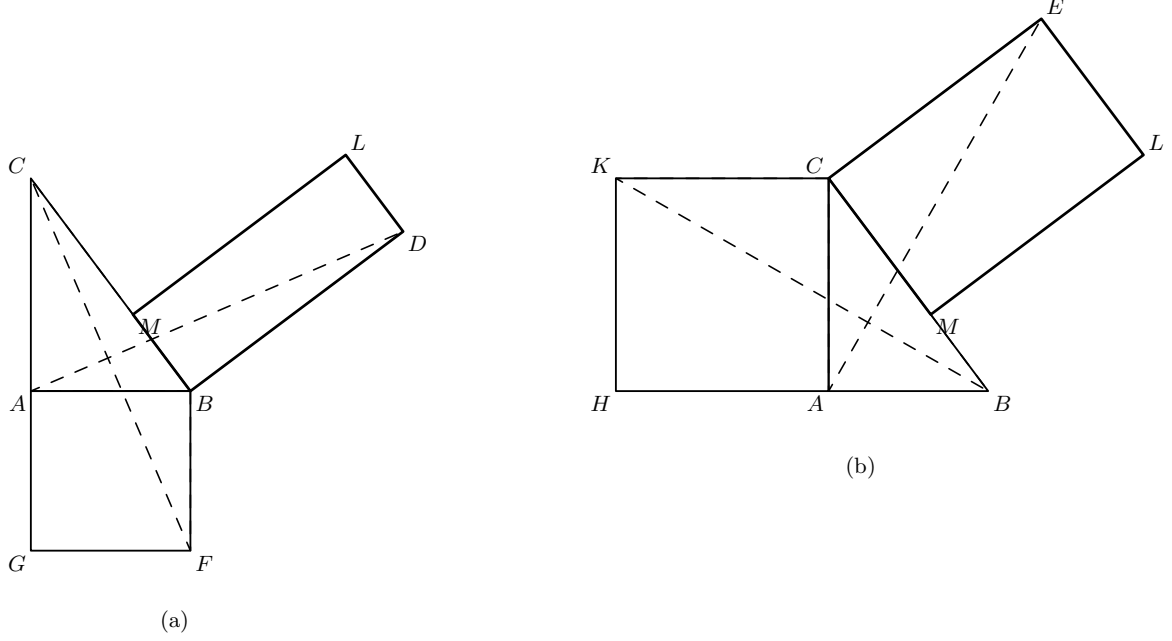
Figure 3: The two symmetric content chains. In panel (a), the dashed triangles BAD and BFC are congruent and connect the square ABFG to the cut parallelogram LDBM via I.41. Panel (b) shows the corresponding triangles CAE and CKB , connecting ACKH to MCEL .
