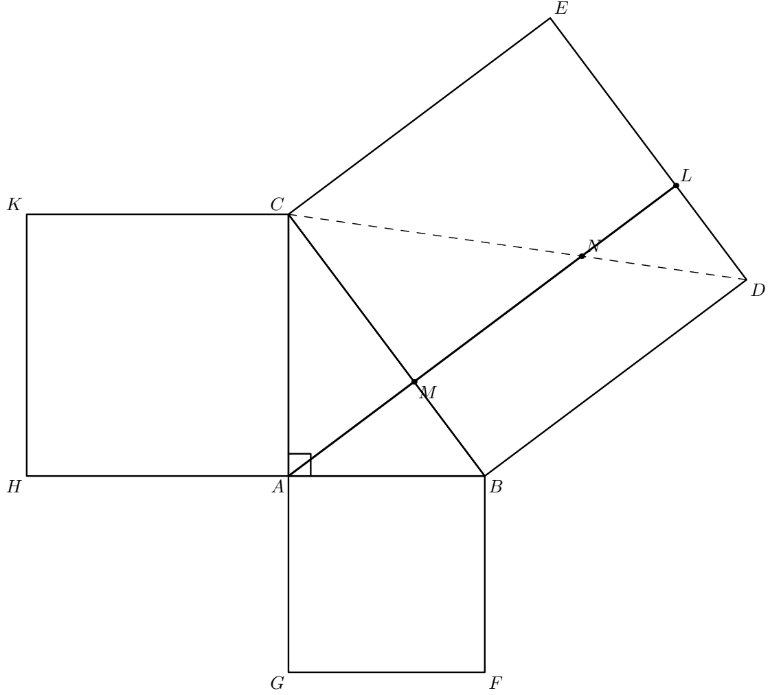
Figure 1: The complete I.47 configuration. The three squares are constructed outward from the right triangle ABC . The line through A, M, L is the internal cut of the square on BC , and the dashed diagonal DC meets it at N . The strict orders used by the scissors proof are B - M - C , D - L - E , D - N - C , and M - N - L .
