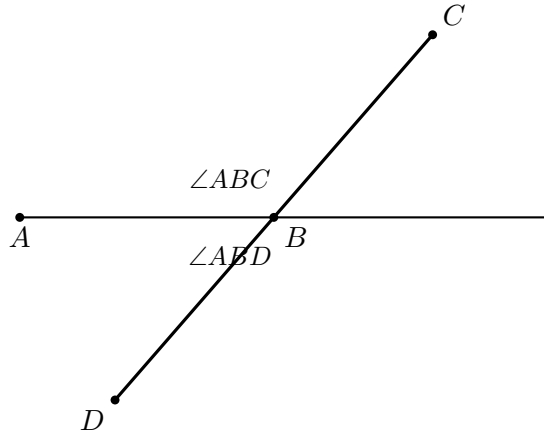
Figure 1: The classical configuration of Proposition I.14. The rays BC and BD lie on opposite sides of the straight line through A and B .
