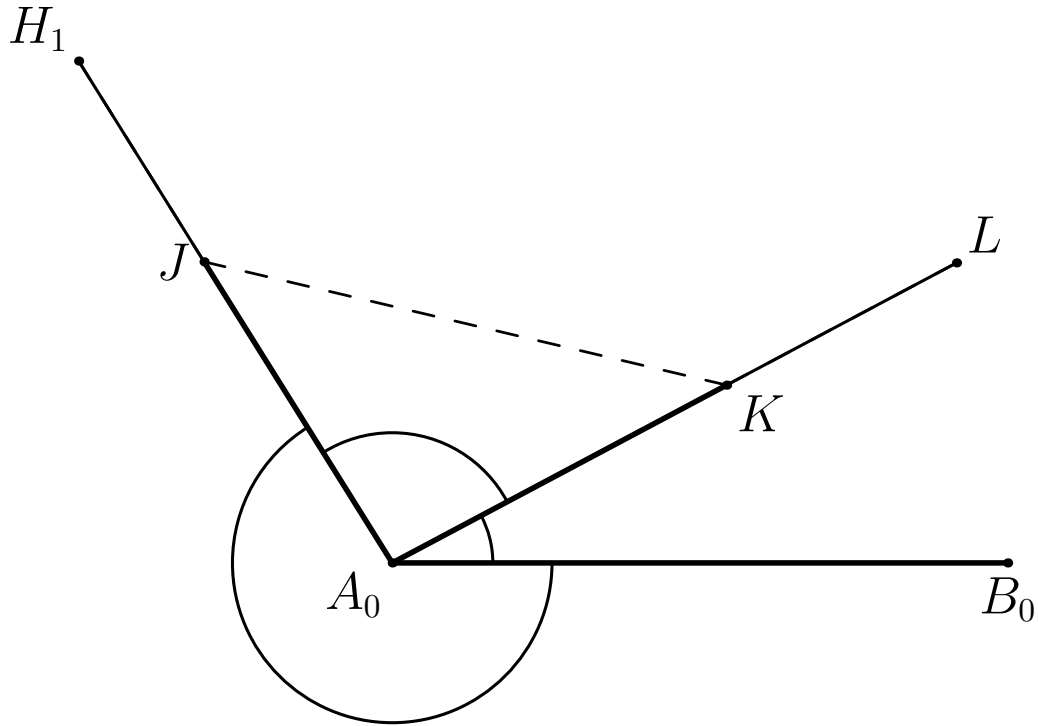
Figure 27.2: The copied trihedral corner at A_0 after the two fourth-proportional constructions. The points K and J lie on the rays copied by XI.26. VI.12 supplies the first two proportions and V.22 supplies the third.
