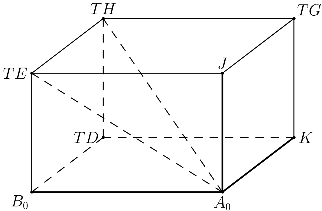
Figure 27.3: The completed target parallelepipedal shell. The three faces incident with A_0 are obtained directly from the scaled corner. Their three opposite faces are recovered by parallel-plane and opposite-edge transport before the final XI.Def.9 packaging.
