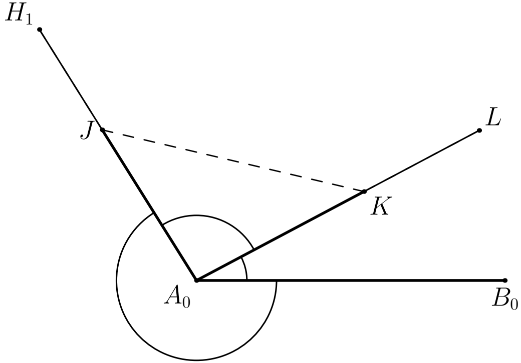
Figure 2: The copied trihedral corner at A_0 after the two fourth-proportional constructions. The points K and J lie on the rays copied by XI.26. VI.12 supplies the first two proportions and V.22 supplies the third.
