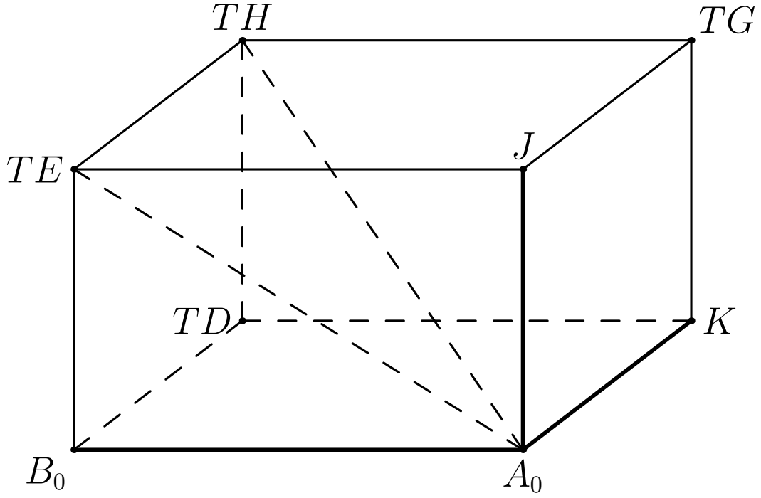
Figure 3: The completed target parallelepipedal shell. The three faces incident with A_0 are obtained directly from the scaled corner. Their three opposite faces are recovered by parallel-plane and opposite-edge transport before the final XI.Def.9 packaging.
