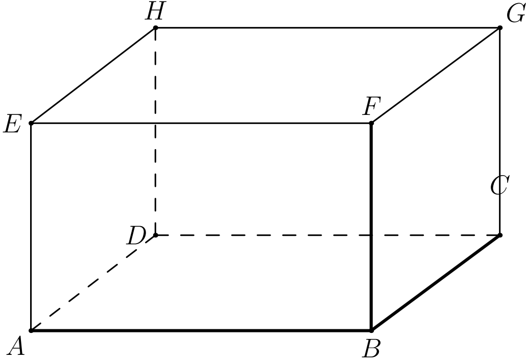
Figure 1: The source parallelepiped and the trihedral corner at B used by the formal construction. The three incident source edges are BA , BC , and BF ; the remaining vertices determine the three opposite faces.
