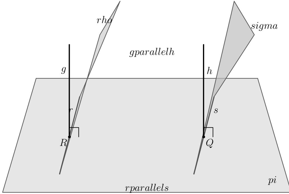
Figure 19.2: The formal incidence step suppressed by the classical picture. If the traces r = \rho \cap \pi and s = \sigma \cap \pi were disjoint, then r \parallel s . Normals g and h to \pi , erected in \rho and \sigma , are parallel by XI.6. XI.15 would then force \rho \parallel \sigma , contradicting the given common point of \rho and \sigma . Therefore the traces meet at the required triple point D .
