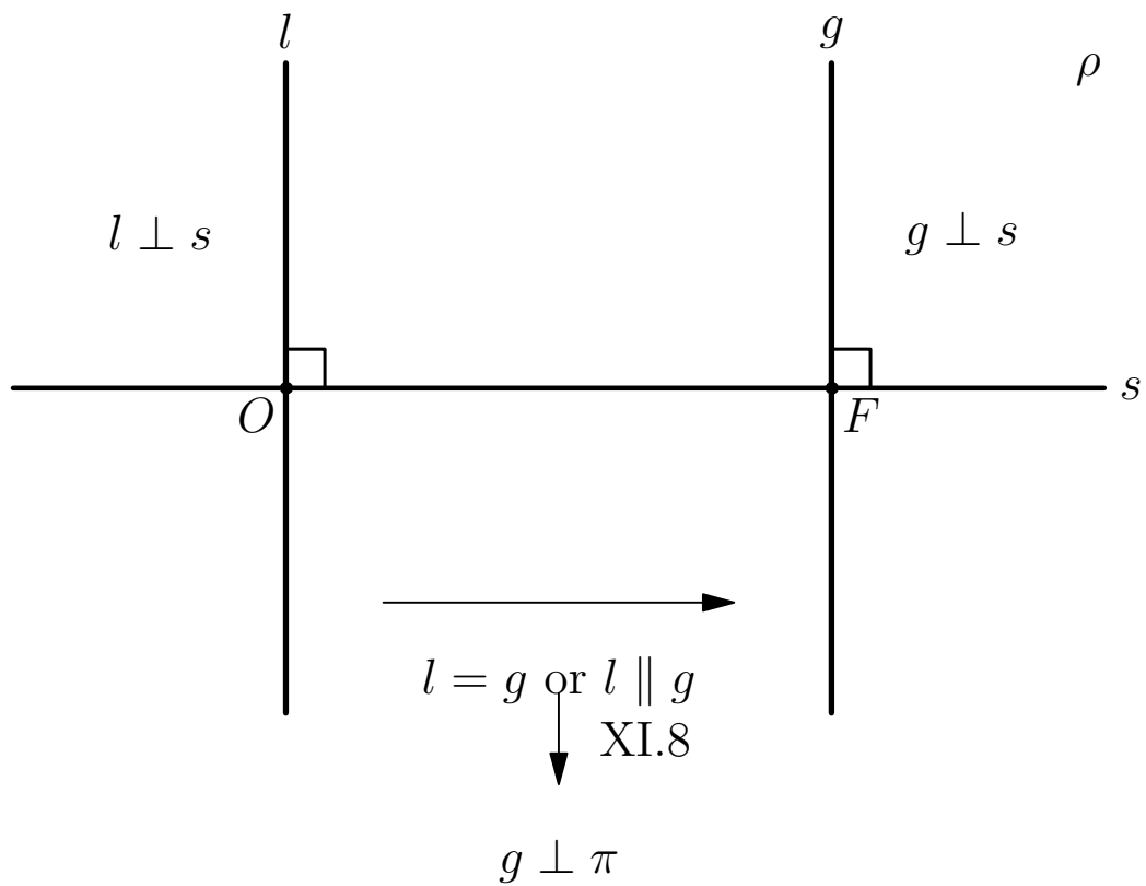
Figure 18.2: The formal core of XI.18 inside the plane \rho . The given normal l and an arbitrary test line g are both perpendicular to the common section s . If their feet coincide then l = g ; if the feet are distinct then the neutral planar argument gives l \parallel g . In the parallel branch XI.8 transports l \perp \pi to g \perp \pi .
