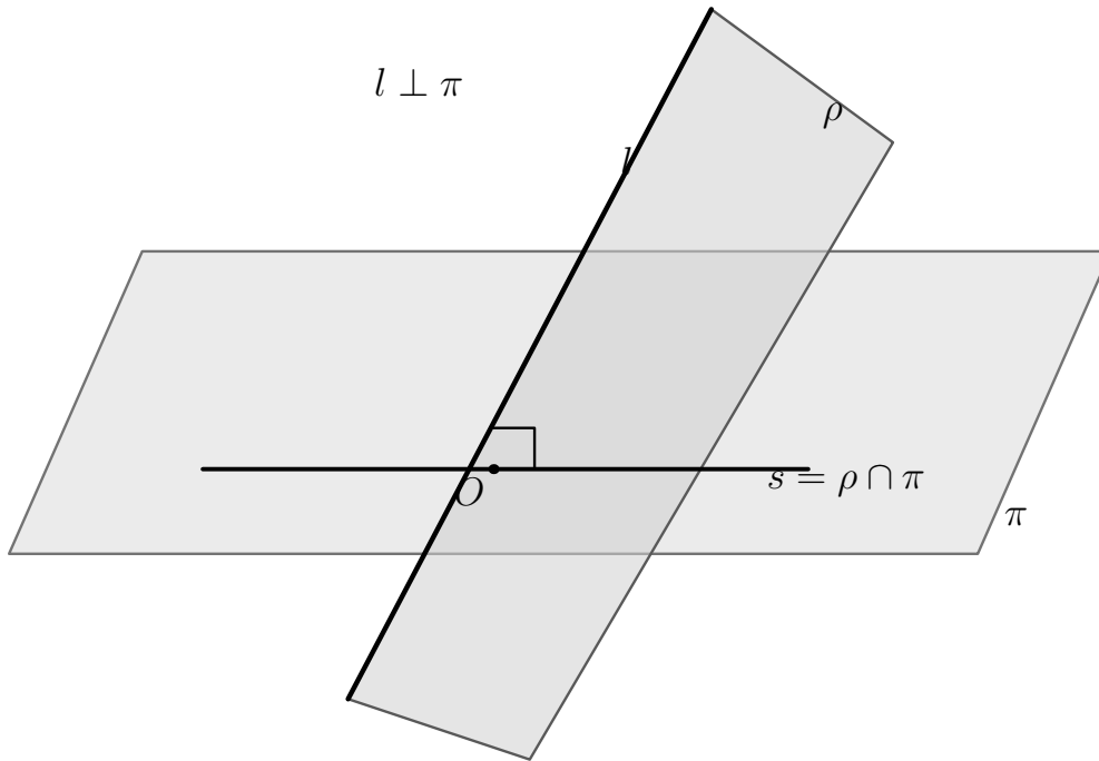
Figure 18.1: The classical configuration of Proposition XI.18. The line l is perpendicular to the reference plane \pi at O , and the arbitrary plane \rho contains l . Its common section with \pi is s = \rho \cap \pi . Proposition XI.18 proves that \rho is perpendicular to \pi in the sense of XI.Def.4.
