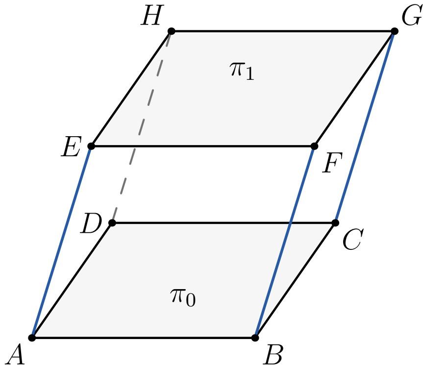
Figure 24.1: Parallelepiped configuration.
