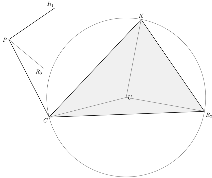
Figure 23.2: The normalized planar core. The three prescribed angles have been copied to one explicit plane. XI.22 produces the base triangle CR_2K ; its circumcenter U and equal radii remain entirely inside \text{PlaneGeo}(\pi) .
