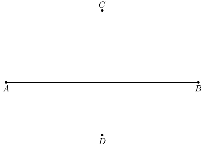
Figure 2: Choose D on the side of the line AB opposite C . This side-of-line information is essential for the later intersection argument.
