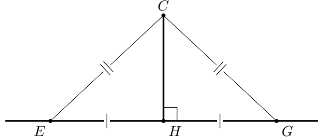
Figure 4: Completed Euclidean proof configuration. The midpoint relation EH \cong HG , the radii CE \cong CG , and the common side CH give SSS for triangles CEH and CGH .
