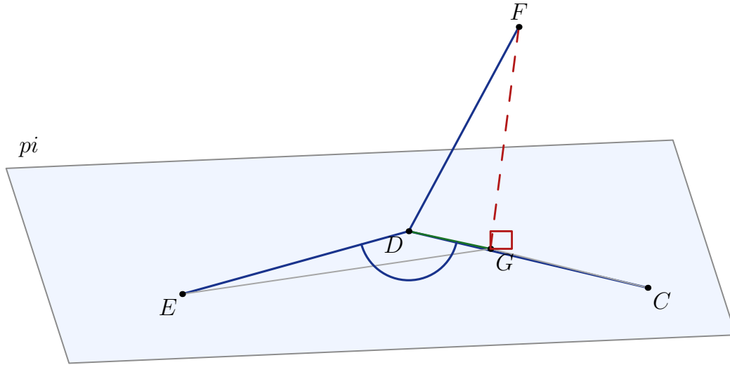
Figure 26.1: The source trihedral angle at D . The point F on the third spatial edge is projected perpendicularly to the base plane \pi through E, D, C , with foot G . The formal proof does not assume any particular order position of G inside that plane.
