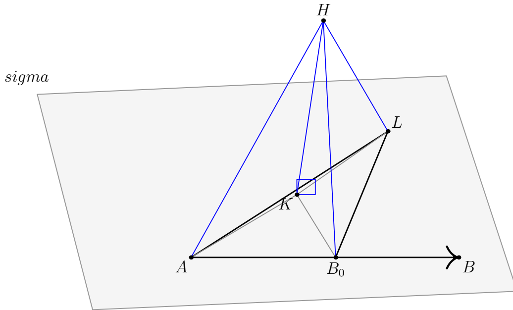
Figure 26.3: The final spatial lift. The points A, B_0, L, K lie in the target base plane, while H is obtained on the perpendicular through K . The three face-angle congruences with the source trihedron are recovered by the shared synthetic metric argument.
