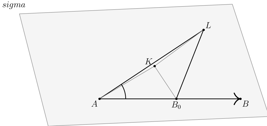
Figure 26.2: The copied planar base at the prescribed point A . The point B_0 lies on the prescribed ray AB , L completes the copied base triangle, and K represents the copied projection point. Metric equalities and angle congruences are stated in the text rather than written on the diagram.
