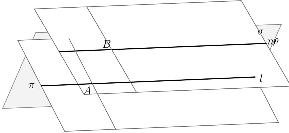
Figure 16.1: A spatial rendering of the configuration of Proposition XI.16. The displayed reference plane is \sigma . The two parallel section lines l = \pi \cap \sigma and m = \rho \cap \sigma lie in \sigma and are drawn in black. The ambient planes \pi and \rho are shown as light auxiliary planes cutting the reference plane along those lines.
