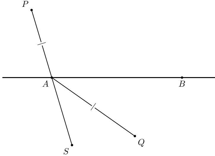
Figure 12.5: Hilbert construction of the reflected point Q . The line PA is extended through A to S ; angle construction chooses the direction of AQ , and segment layoff gives AQ \cong AP .
