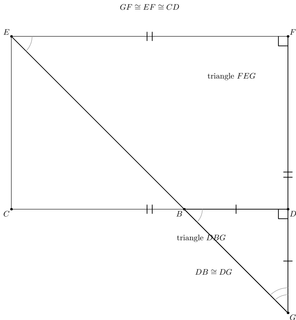
Figure 4: Once the orders E - B - G and F - D - G are known, the source angle argument acts on two visible triangles. In DBG , the vertical-angle and right-angle chain makes the angles at B and G congruent, so I.6 yields DB \cong DG . In FEG , the corresponding half-right-angle argument and the right angle at F give GF \cong EF ; I.34 then transports the latter length to CD . Local angle-decomposition witnesses are omitted.
