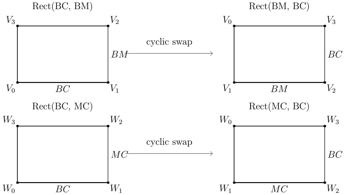
Figure 2: The two independent representative changes performed in Step 2. The first changes the presentation of a rectangle contained by BC, BM to one contained by BM, BC ; the second does the same for BC, MC . The quadrilateral is not replaced by a new metric figure: its vertices are cyclically re-indexed, and rectangle_contained_by_swap supplies the exact scissors certificate for that re-presentation.
