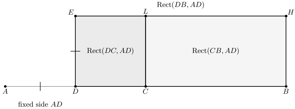
Figure 3: The second formal dissection. The derived order D - C - B allows the binary II.1 theorem to cut the rectangle contained by DB, AD into the two visible pieces contained by DC, AD and CB, AD . The small segment AD at the left records the fixed second-side magnitude. The subsequent replacement of \text{Rect}(DC, AD) by \text{Rect}(AD, DC) is a rotation/contained-by normalization of a representative, so it receives no additional geometric picture.
