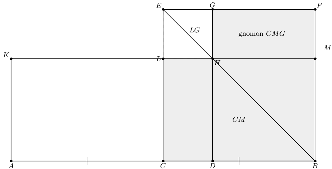
Figure 1: The classical configuration of Euclid II.5. The square CEFB is built on the half CB in the customary mirror orientation A - C - D - B . The diagonal BE and the parallels through the unequal cut D form the complementary-parallelogram configuration; LG is the small square on CD , and the shaded remainder is Euclid's gnomon. This figure is retained because it is the actual source geometry. The later formal figures use the Lean orientation A - D - C - B and do not introduce a primitive gnomon object.
