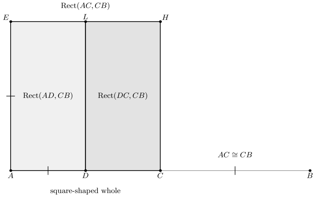
Figure 4: The final geometric assembly used by the reconstruction. After cyclically rotating the two incoming representatives, II.1 reads the order A - D - C as an actual cut of a rectangle with common side magnitude CB : the two pieces contained by AD, CB and DC, CB fill the rectangle contained by AC, CB . The congruence AC \cong CB marks its adjacent side magnitudes as equal, explaining the final square recognition. Lean may compare this whole with a different supplied square representative by uniqueness; that representative bookkeeping does not create another spatial state.
