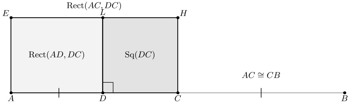
Figure 2: The first formal dissection in II.5, shown in the Lean orientation A - D - C - B . Proposition II.3 cuts the rectangle contained by AC, DC at D into a rectangle contained by AD, DC and a square-shaped DC piece. The continuation to B and the matching marks record the independent midpoint fact AC \cong CB , which transports the whole rectangle to one contained by CB, DC . The separately supplied square and rectangle representatives used by Lean are deliberately omitted: they do not change this geometric cut.
