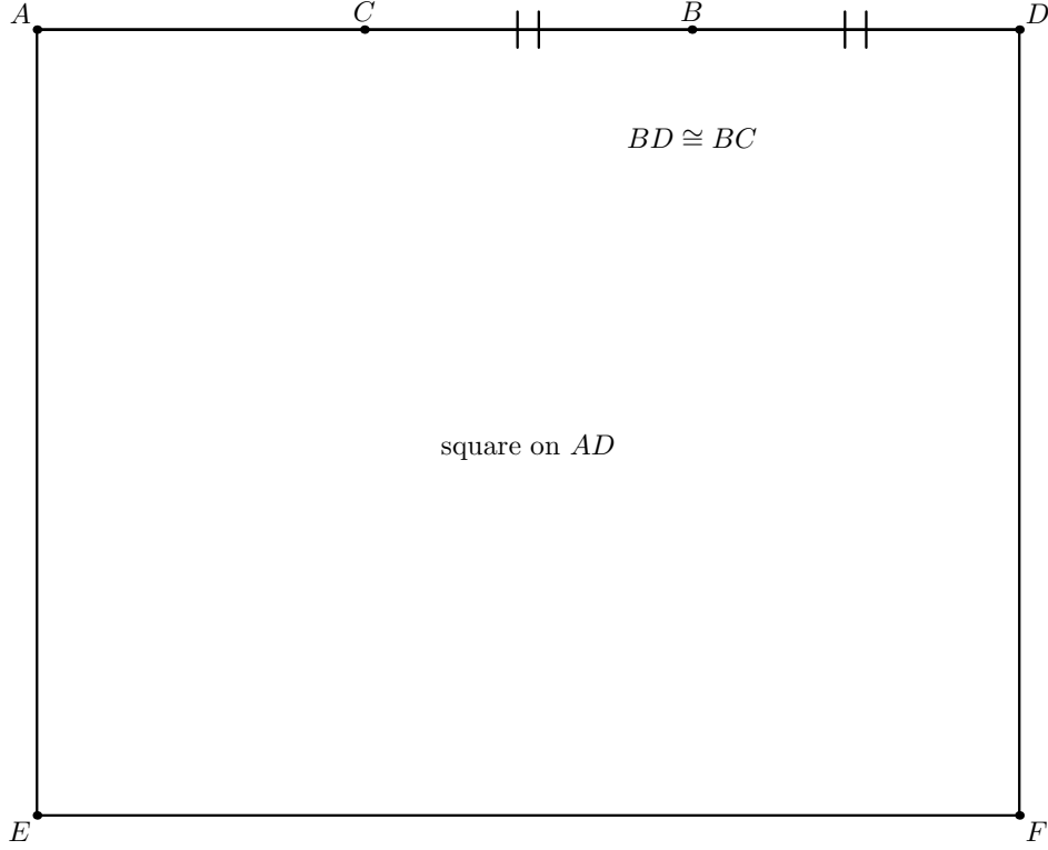
Figure 1: The initial geometric state for Proposition II.8. The order is A - C - B - D , the produced segment satisfies BD \cong BC , and the square on AD has been constructed. No II.4 or II.7 subdivision is shown yet. In particular, the figure records the geometry that makes the later representative transports meaningful without pretending that the Lean proof reconstructs Euclid's full eight-region gnomon.
