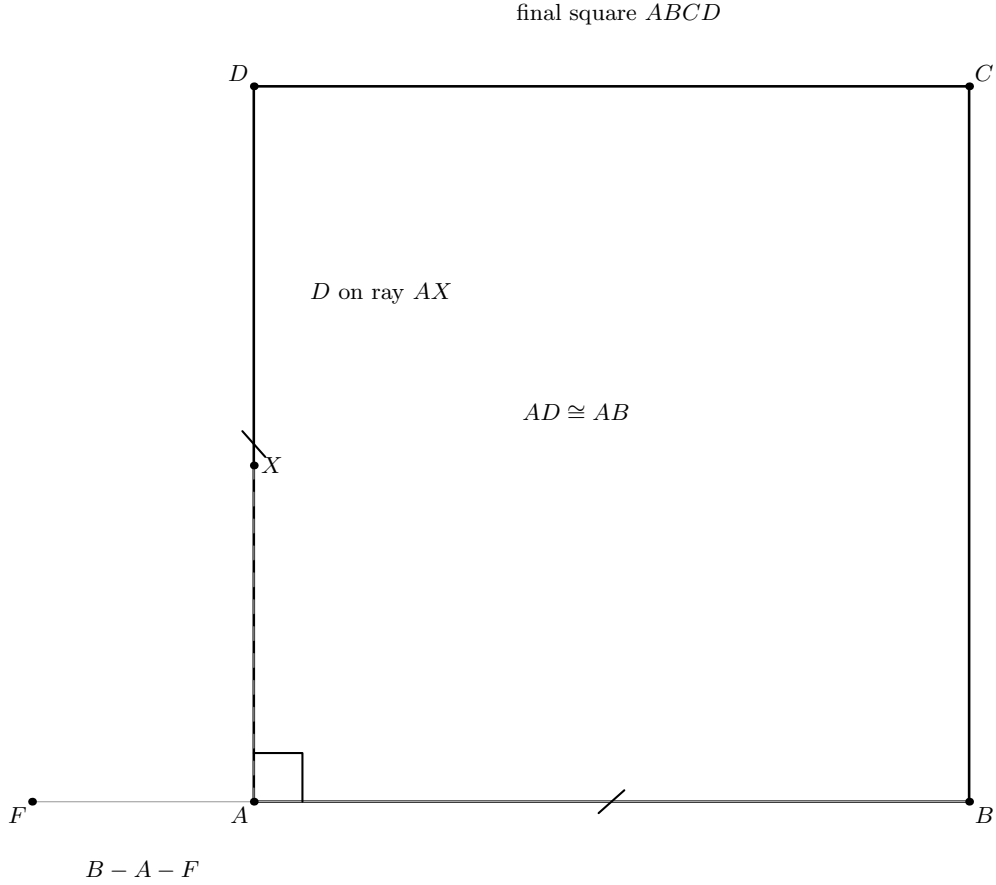
Figure 1: The square ABCD on the given segment AB . The auxiliary point F satisfies B - A - F , allowing the right-angle construction at the endpoint A . The point X determines the perpendicular ray, and D is laid off on that ray with AD \cong AB . The fourth vertex C is then obtained by completing the parallelogram.
