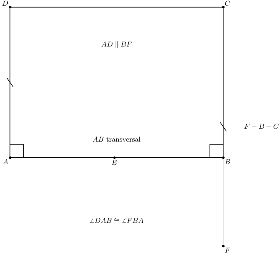
Figure 2: The reusable I.29 configuration extracted from Proposition I.46. The side CB is extended through B to F , so F - B - C . The side AB acts as a transversal of the parallel carriers AD and BF . The Euclidean alternate-angle theorem gives \angle DAB \cong \angle FBA . If \angle DAB is right, rightness transfers to \angle FBA and then across the straight extension F - B - C to \angle ABC .
