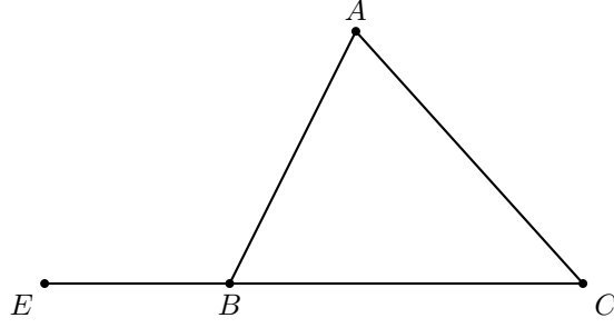
Figure 2: The second extension used by the Lean wrapper: CB is produced beyond B .
