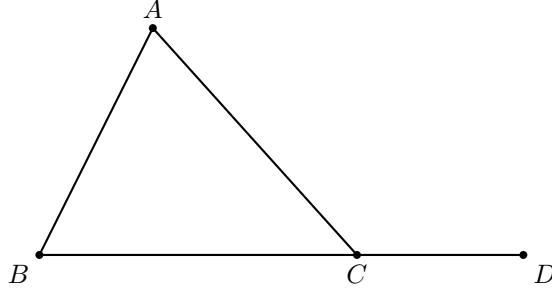
Figure 1: The classical extension used for the pair \angle ABC, \angle ACB : BC is produced beyond C .
