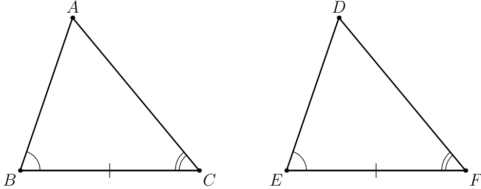
Figure 1: The common input configuration for Proposition I.26. The two pairs of corresponding angles are marked by one and two arcs respectively, and in the ASA case the corresponding side BC \cong EF is marked by a single tick.
