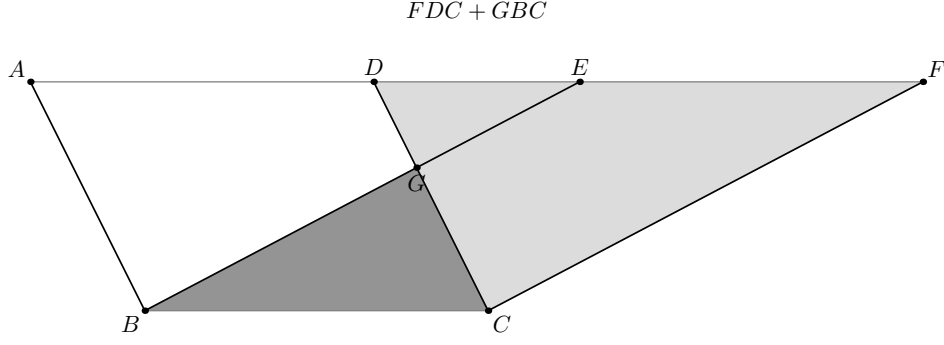
Figure 7: Step 3. Replace the congruent outer triangle: EAB + GBC \sim FDC + GBC .
