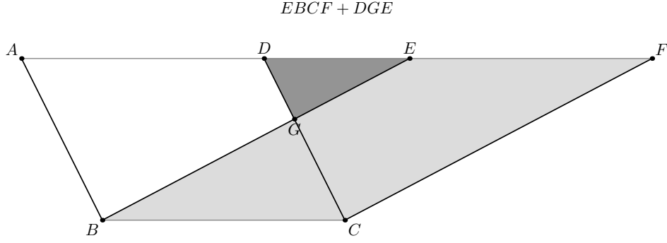
Figure 8: Step 4. Regroup the pieces as the second augmented parallelogram EBCF + DGE .
