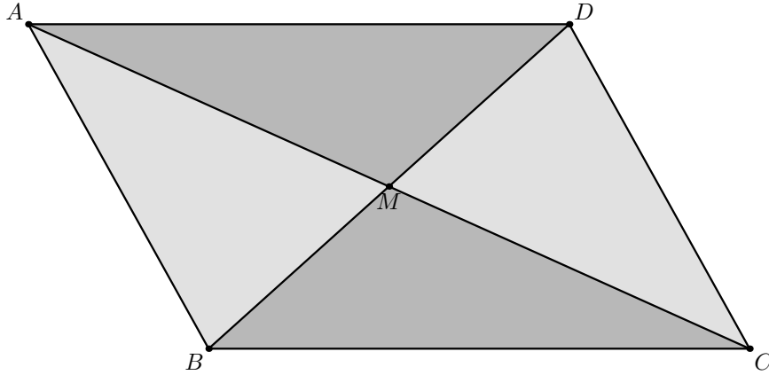
Figure 3: Common refinement at the diagonal intersection M .
