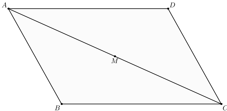
Figure 2: First triangulation of the quadrilateral, along the diagonal AC .
