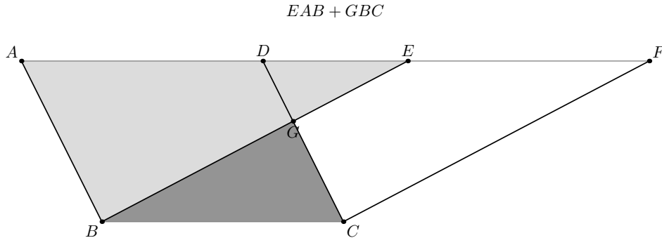
Figure 6: Step 2. The augmented left-hand figure is rearranged as EAB + GBC .
