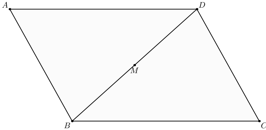
Figure 4: Second triangulation of the same quadrilateral, along the diagonal BD .
