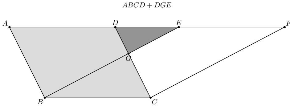
Figure 5: Step 1. Adjoin the triangle DGE to the parallelogram ABCD .
