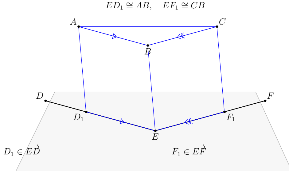
Figure 10.6: Wrapper-level segment construction. Only the points D_1 and F_1 are laid off on the rays ED and EF , with ED_1 \cong AB and EF_1 \cong CB . This yields the normalized configuration used by the internal core theorem.
