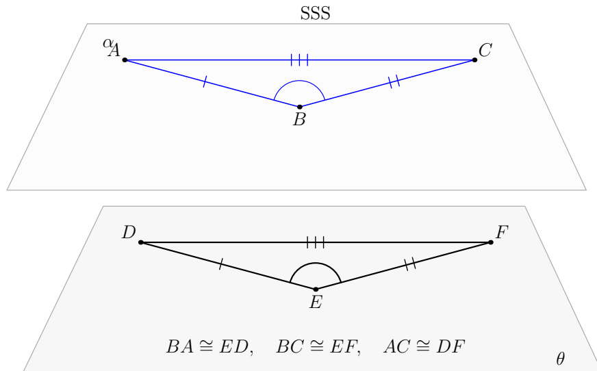
Figure 10.5: The final normalized SSS state. The three pairs of corresponding sides are marked separately: BA \cong ED , BC \cong EF , and AC \cong DF . The two triangles lie in distinct parallel plane slices.
