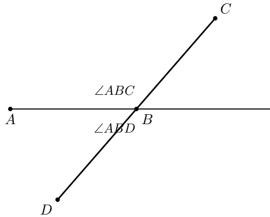
Figure 14.1: The classical configuration of Proposition I.14. The rays BC and BD lie on opposite sides of the straight line through A and B .
