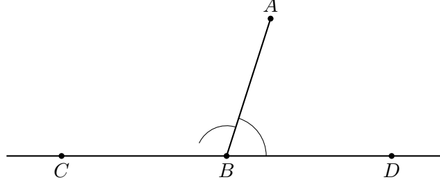
Figure 13.1: Configuration of Proposition I.13. The point B lies between C and D , and the ray BA forms the adjacent angles \angle CBA and \angle ABD with the straight line CD .
