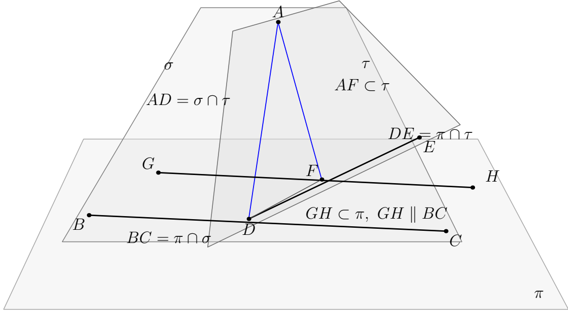
Figure 2: The three plane slices used by the reconstruction. The reference plane \pi contains BC, DE, GH . The plane \sigma carries the first planar perpendicular construction and shares BC with \pi . The plane \tau carries AD, DE, AF ; it shares AD with \sigma and DE with \pi . The final argument transfers perpendicularity from BC to GH through XI.8 and then applies XI.4 in \pi .
