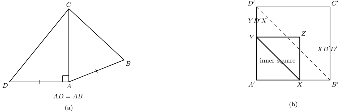
Figure 1: Two geometric layers of the I.48 reconstruction. Panel (a) shows the auxiliary right triangle: AD \cong AB and \angle DAC is right, while the original angle BAC is not assumed right in the drawing. Panel (b) shows the proper-part configuration used to prove monotonicity of square content. If a side is strictly shorter, points X and Y cut equal initial parts from two adjacent sides of the larger square, producing the inner square A'XZY . In one diagonal half the remainder is the pair of nondegenerate triangles YD'X and XB'D' ; the square argument produces two copies of that pair.
