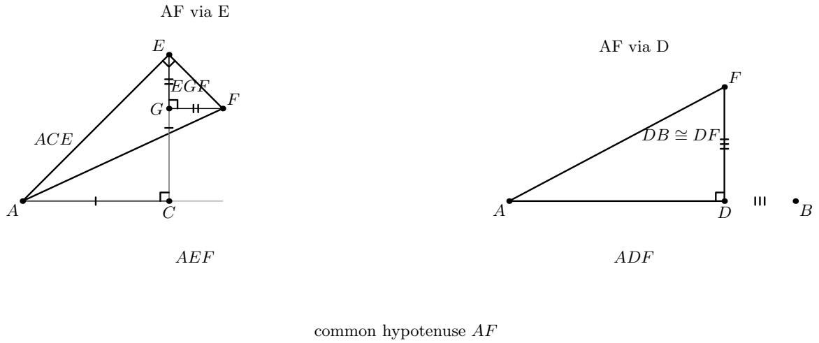
Figure 6: The four right triangles used by I.47, organized by the common square on AF . The left panel follows AF through the right triangle AEF , then expands its two leg squares with the right triangles ACE and EGF . The right panel gives the independent decomposition of the same hypotenuse through ADF . Segment congruences later transport DF to DB , the two A/C/E legs to AC , and GE, GF to CD . No literal square representatives are drawn because the formal proof may construct them independently and then transport their content.
