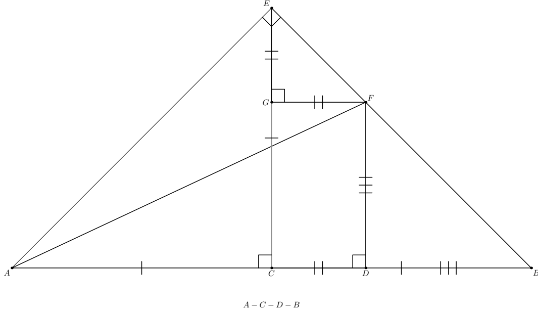
Figure 1: The source-faithful configuration for Proposition II.9 in the oriented branch A-C-D-B . The perpendicular CE is copied from the half of AB ; DF \parallel CE and FG \parallel CD form the parallelogram DFGC with E-F-B and C-G-E . Euclid's angle argument gives GE = GF and DF = DB , while I.34 gives GF = CD . The four right triangles used by I.47 are ACE , EGF , AEF , and ADF . The auxiliary I.32 witnesses used by Lean are omitted from the drawing to keep the classical mechanism visible.
