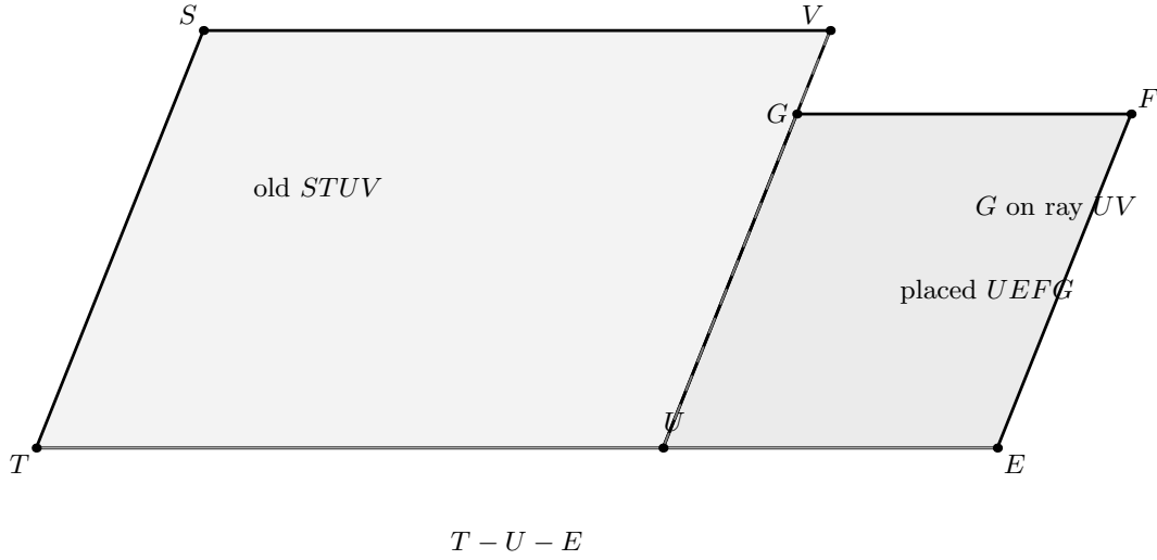
Figure 2: The orientation step used before the I.44 positioned construction. The old parallelogram is STUV . The base carrier is produced to E , giving T - U - E , while G is laid off on the old ray UV . Completing U, E, G gives the auxiliary parallelogram UEFG , which has the content of the new triangle. The explicit ray choice is the information not retained by the public I.44 wrapper.
