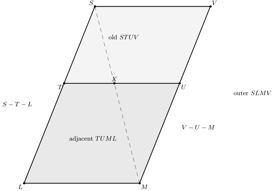
Figure 1: Two adjacent parallelograms in the exact order configuration used by the Lean proof. The old parallelogram is STUV , the new one is TUML , and the strict relations S - T - L and V - U - M put the new piece outside the old one. Their outer boundary is the parallelogram SLMV . The dashed segment SM meets the common side TU at X , giving S - X - M and T - X - U for the scissors refinement.
