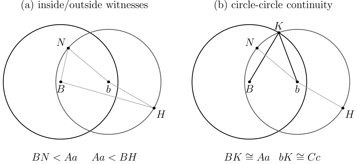
Figure 5: Formal circle-continuity chain. Both N and H lie on the circle centered at b with radius congruent to Cc . In the strict-inside branch, BN < Aa while Aa < BH ; circle-circle continuity then supplies a common point K , after which congruence transport yields BK \cong Aa and bK \cong Cc .
