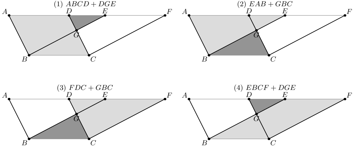
Figure 5: The exact four-stage scissors witness in the disjoint case. The formal proof passes from ABCD + DGE to EAB + GBC , replaces the congruent outer triangle, and regroups to EBCF + DGE . The nonzero complement is the same geometric triangle DGE on both sides.
