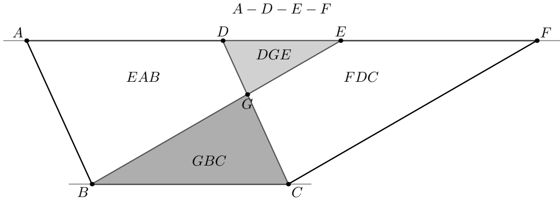
Figure 2: The classical disjoint configuration of Proposition I.35. The outer triangles EAB and FDC are compared. Their crossing sides determine G ; Euclid subtracts the common triangle DGE and then adds the common triangle GBC .
