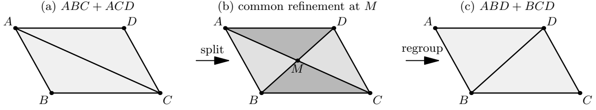
Figure 3: The generic diagonal-flip lemma used by the I.35 scissors layer. The two diagonal triangulations pass through one common four-triangle refinement at the internal intersection point M .
