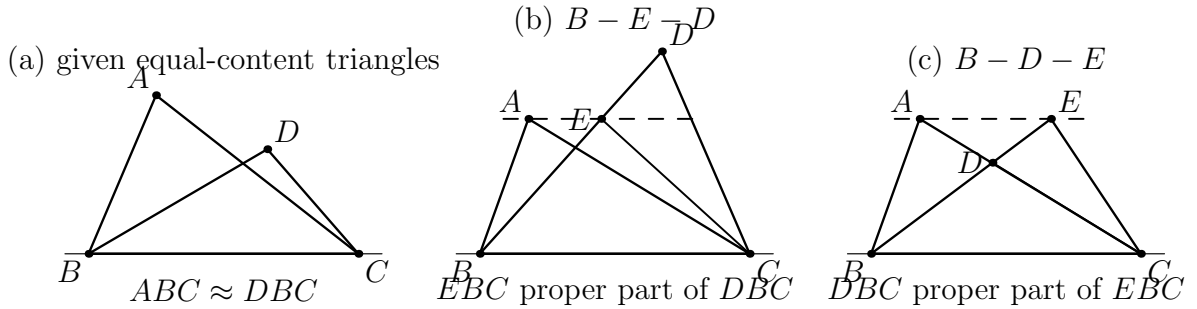
Figure 1: The geometric configuration used in the reconstruction of I.39. (a) The given triangles ABC and DBC share the base BC , lie on the same side of its carrier, and are assumed equicomplementable. (b) The parallel through A meets BD at E with B - E - D ; Proposition I.37 gives equal content for ABC and EBC , while EBC is a proper subtriangle of DBC . (c) The alternative order is B - D - E ; now DBC is a proper subtriangle of EBC . The order E - B - D is excluded formally because it would put E and D on opposite sides of the base.
