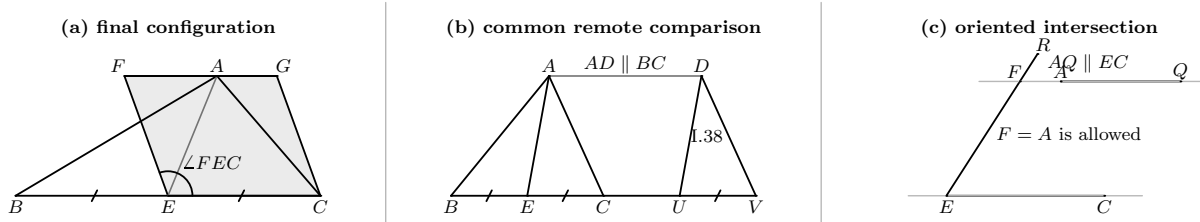
Figure 1: Three geometric stages of I.42. (a) The final configuration: E is the midpoint of BC , the upper carrier contains F, A, G , and FECG is the required parallelogram. (b) The formal proof that the median halves have equal content does not appeal to numerical altitude: both ABE and AEC are compared by I.38 with one remote triangle DUV , where BE \cong EC \cong UV and the upper carrier through A, D is parallel to the common base carrier. (c) The copied angle ray ER is proved to meet the parallel AQ at F ; SameSide information then selects the correct ray. The special case F = A is valid and is handled explicitly.
