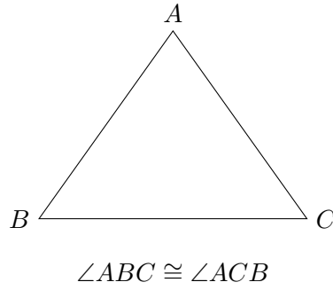
Figure 1: The initial triangle with equal base angles.
