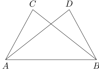
Figure 1: The assumed existence of two distinct vertices on the same side of the base AB .
