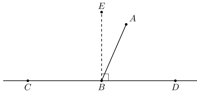
Figure 2: Euclid's auxiliary construction in the second case. By Proposition I.11 the perpendicular BE is erected at B on the straight line CD .
