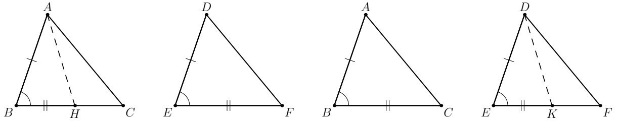
(a) Assume EF < BC : choose B - H - C with BH \cong EF .
