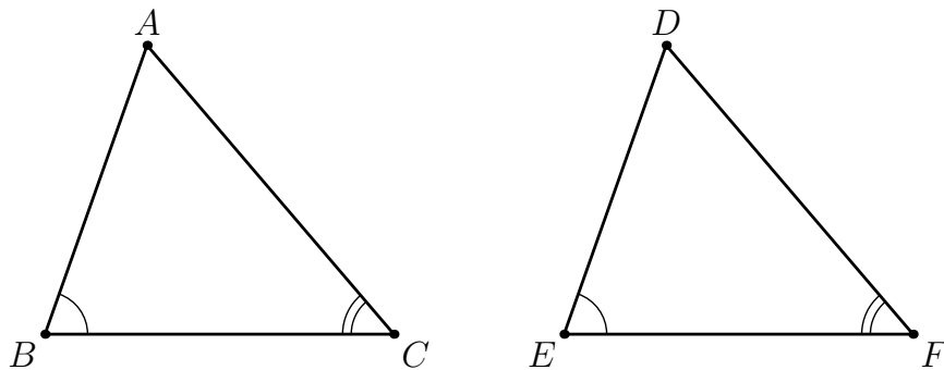
Figure 1: The common angle data of Proposition I.26: \angle ABC \cong \angle DEF and \angle BCA \cong \angle EFD . No side congruence is marked: the ASA clause assumes BC \cong EF , whereas the SAA clause assumes AB \cong DE .
