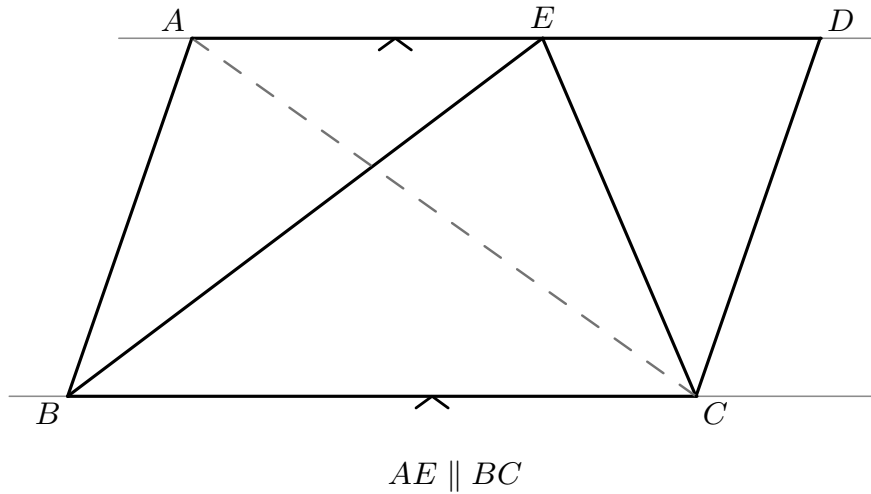
Figure 1: The classical I.41 configuration. The parallelogram ABCD and triangle EBC have the common base BC and lie between the same parallel carriers. Euclid joins the auxiliary diagonal AC , which is the diagonal consumed by I.34. The displayed placement of E on the upper carrier is representative only: the formal theorem assumes AE \parallel BC and does not assume a betweenness order among A, D, E .
