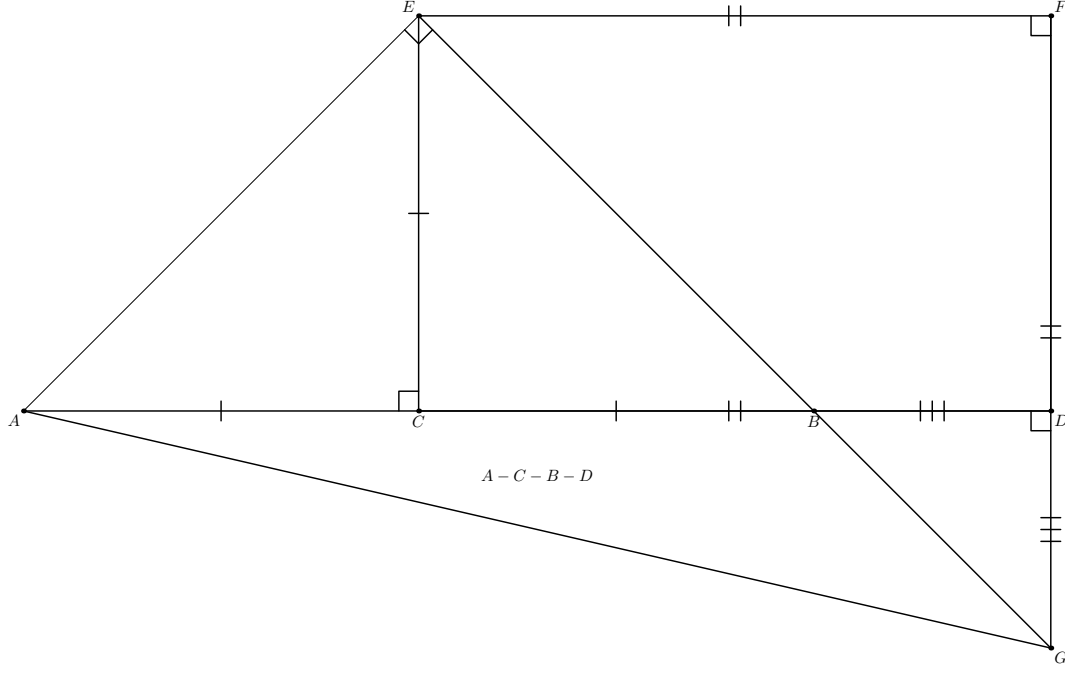
Figure 1: The source-faithful configuration for Proposition II.10 in the order A - C - B - D . The segment CE is perpendicular to the base and satisfies CE = AC = CB . The quadrilateral CDFE is a parallelogram, while the produced lines satisfy E - B - G and F - D - G . Euclid's angle argument gives DB = DG and GF = EF ; I.34 gives EF = CD . The four right triangles used by I.47 are ACE , FEG , EAG , and DAG . Auxiliary interior-ray witnesses used by Lean are omitted from the drawing.
