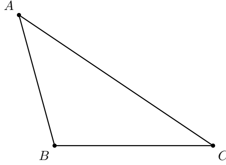
Figure 1: Classical configuration for Proposition I.19. The hypothesis is \angle ACB < \angle ABC ; the conclusion is AB < AC .
