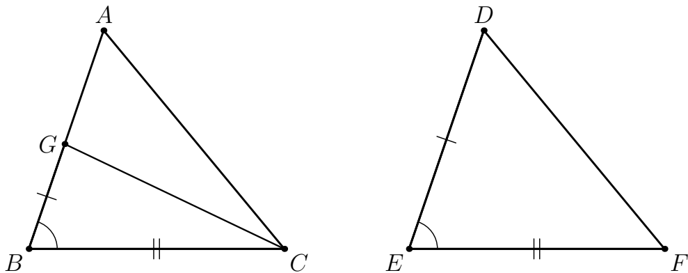
Figure 2: Euclid's ASA reductio configuration. The point G lies between A and B . The diagram marks exactly the local SAS data GB \cong DE , BC \cong EF , and \angle GBC \cong \angle DEF .
