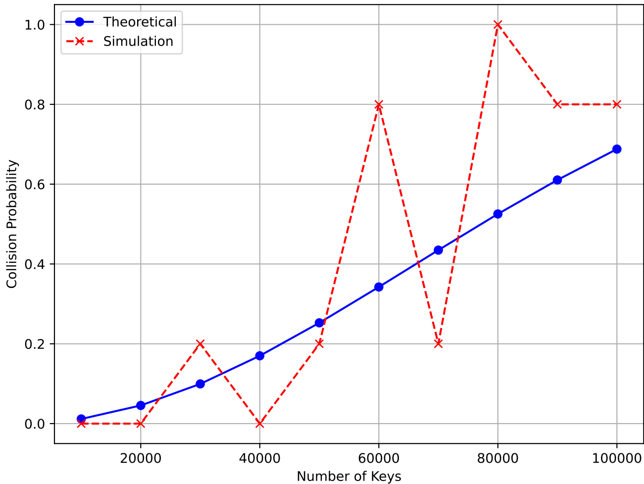
Collision Probability vs Number of Keys (32-bit truncated hash)
